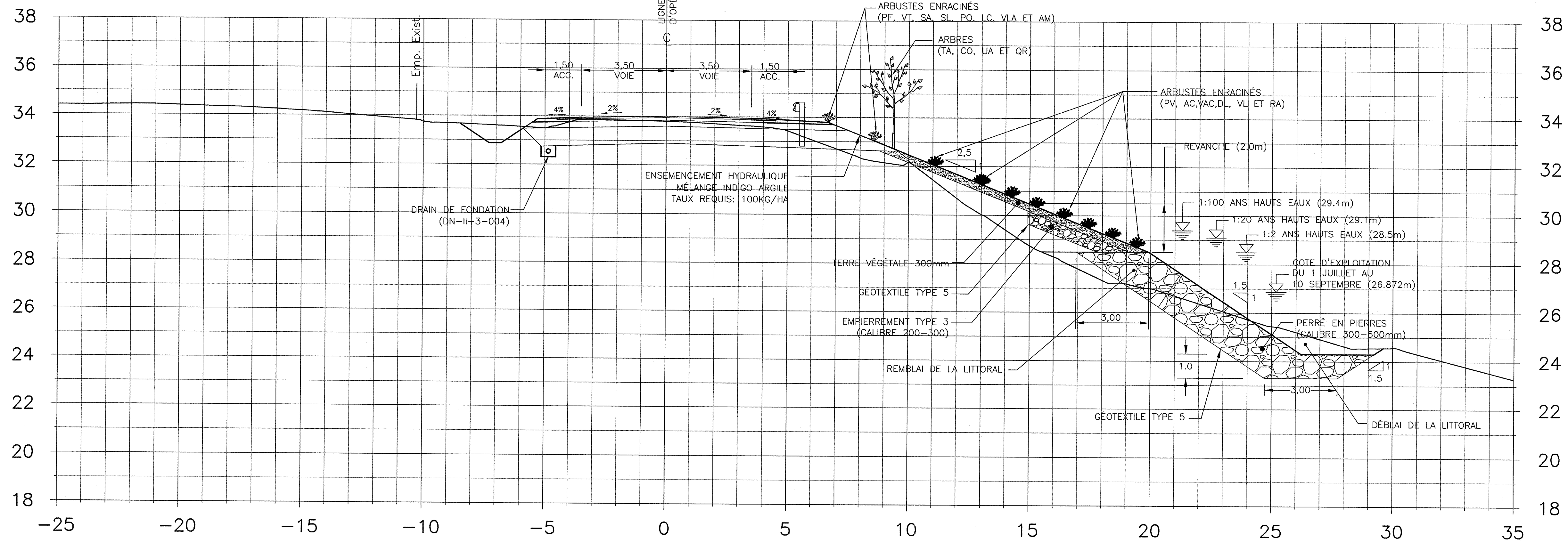
ROUTE 231 COUPE TRANSVERSALE CH. 2+240
