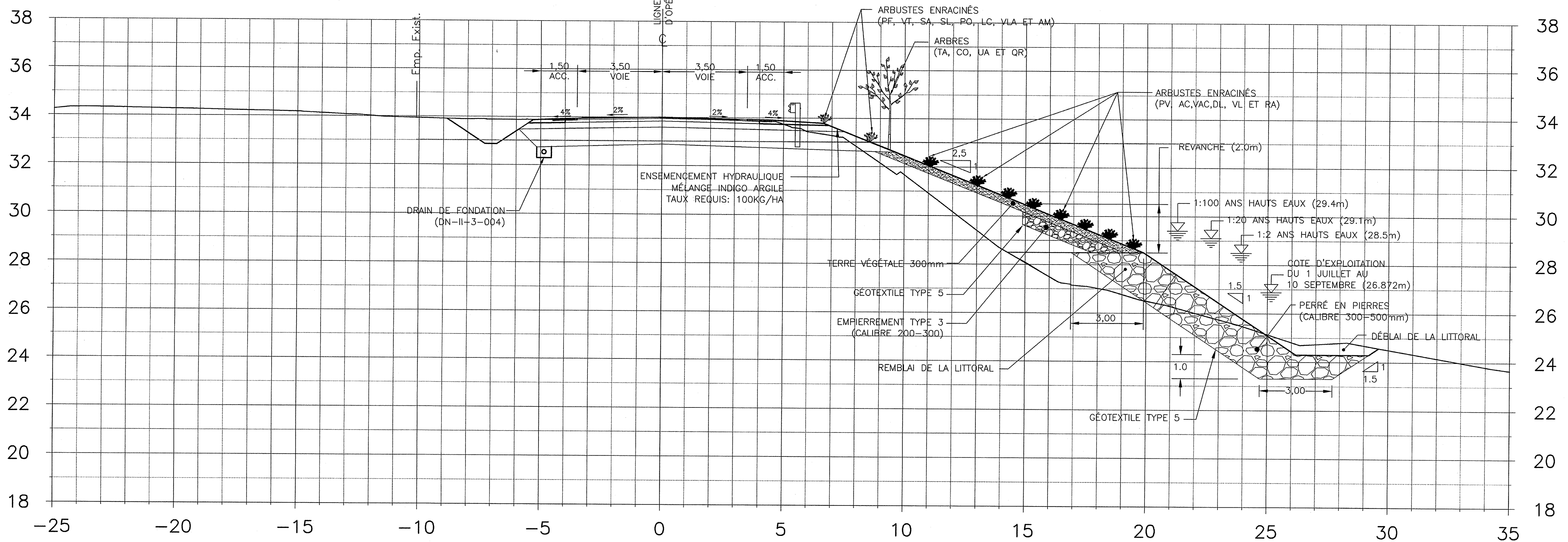
ROUTE 231 COUPE TRANSVERSALE CH. 2+280
