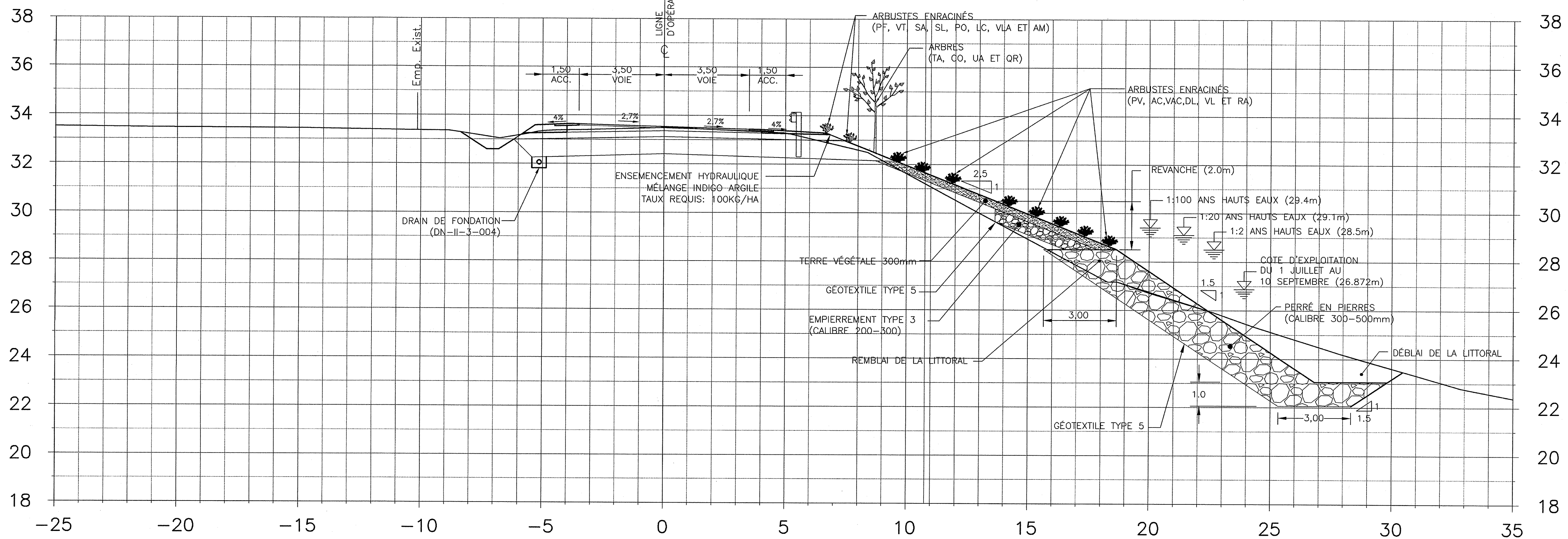
ROUTE 231 COUPE TRANSVERSALE CH. 1+580
