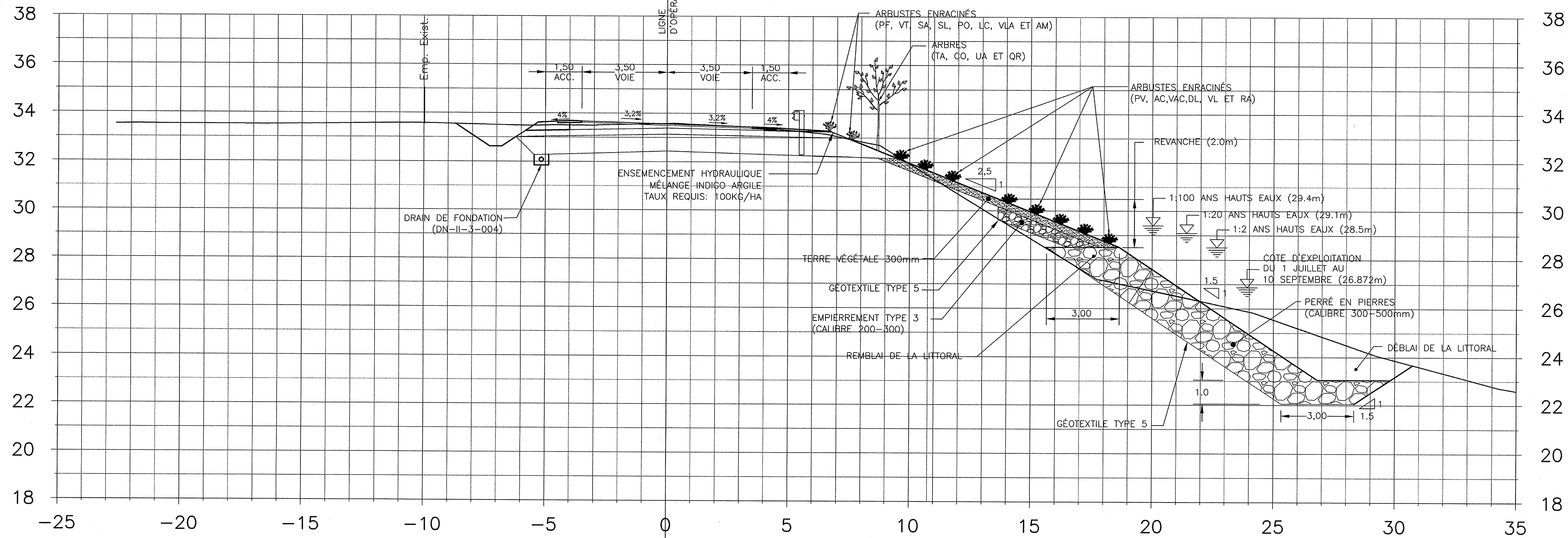
ROUTE 231 COUPE TRANSVERSALE CH. 1+540
