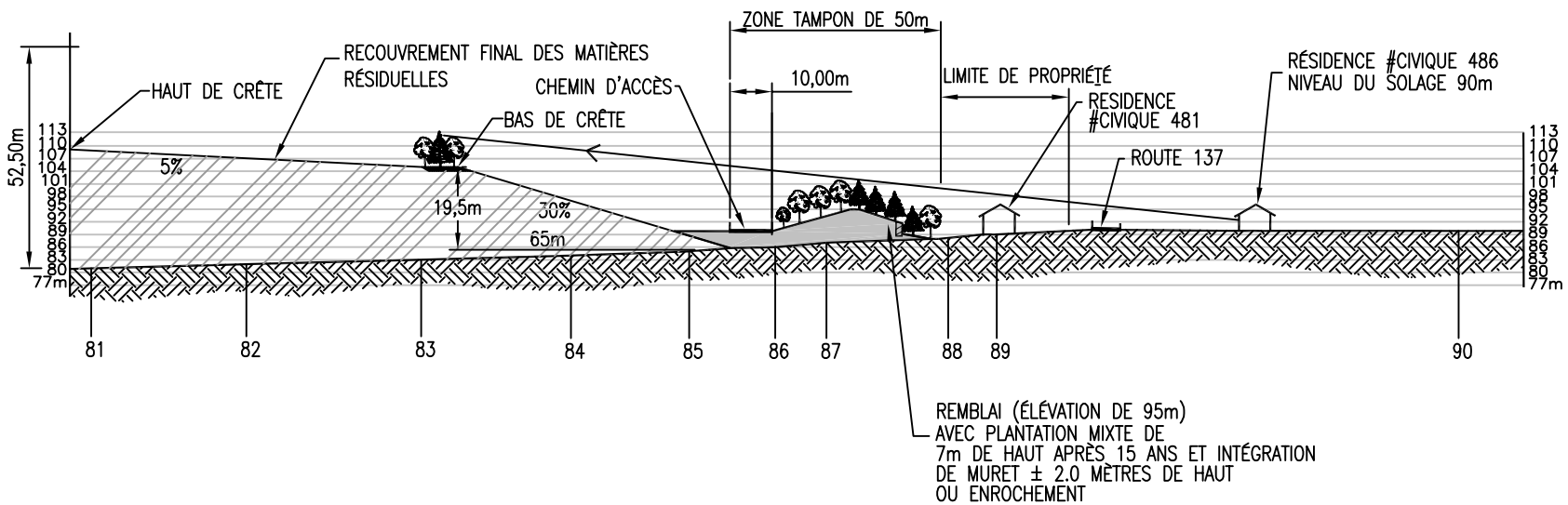
Figure 4.8: Coupe C-C
