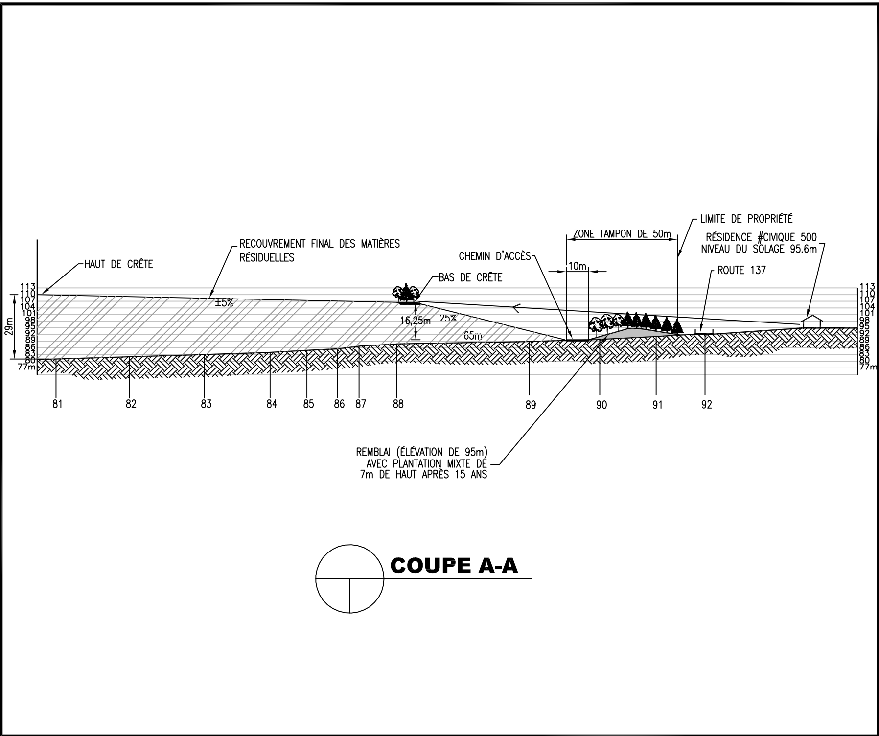
Figure 4.6: Coupe A-A
