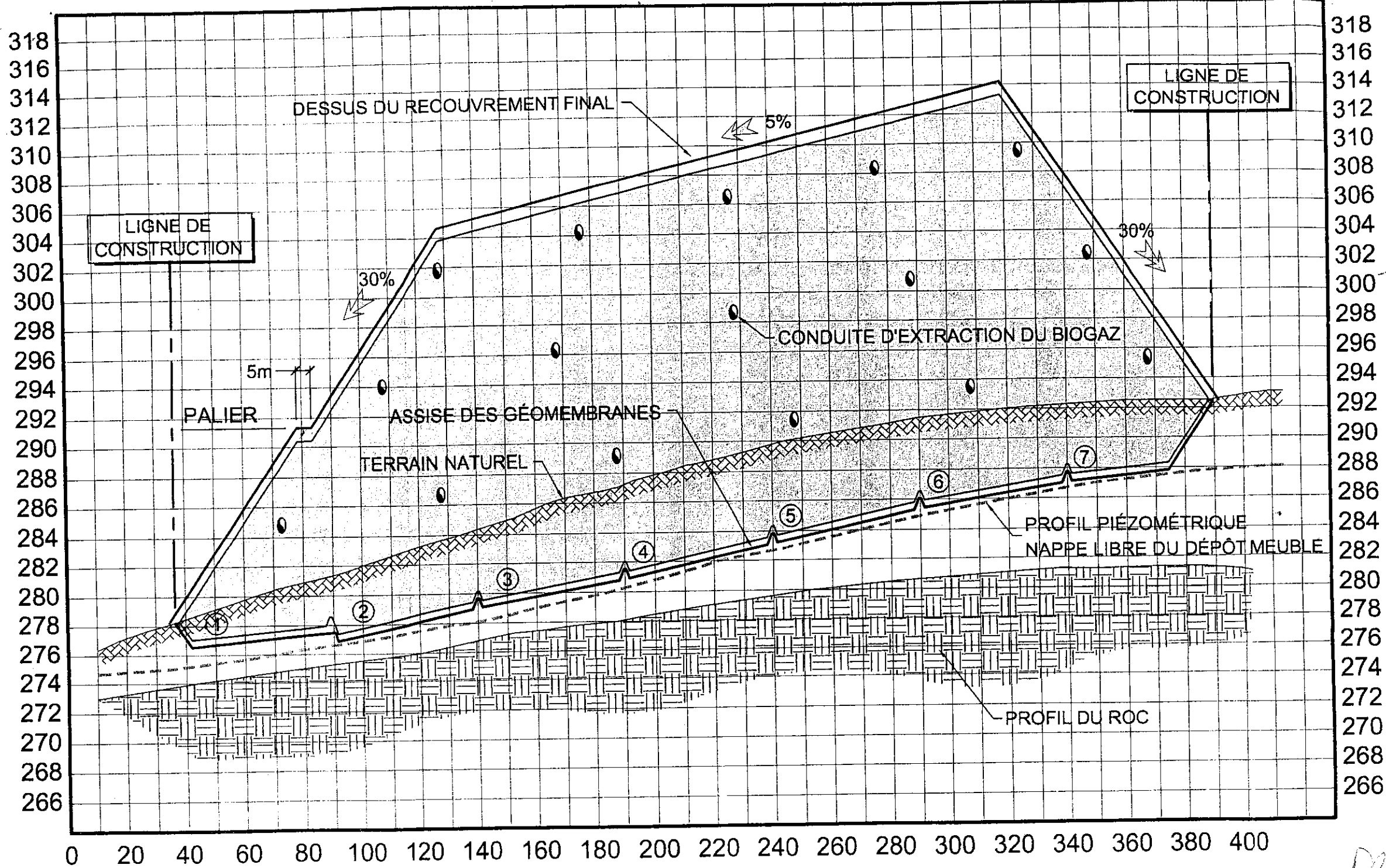
SECTION
