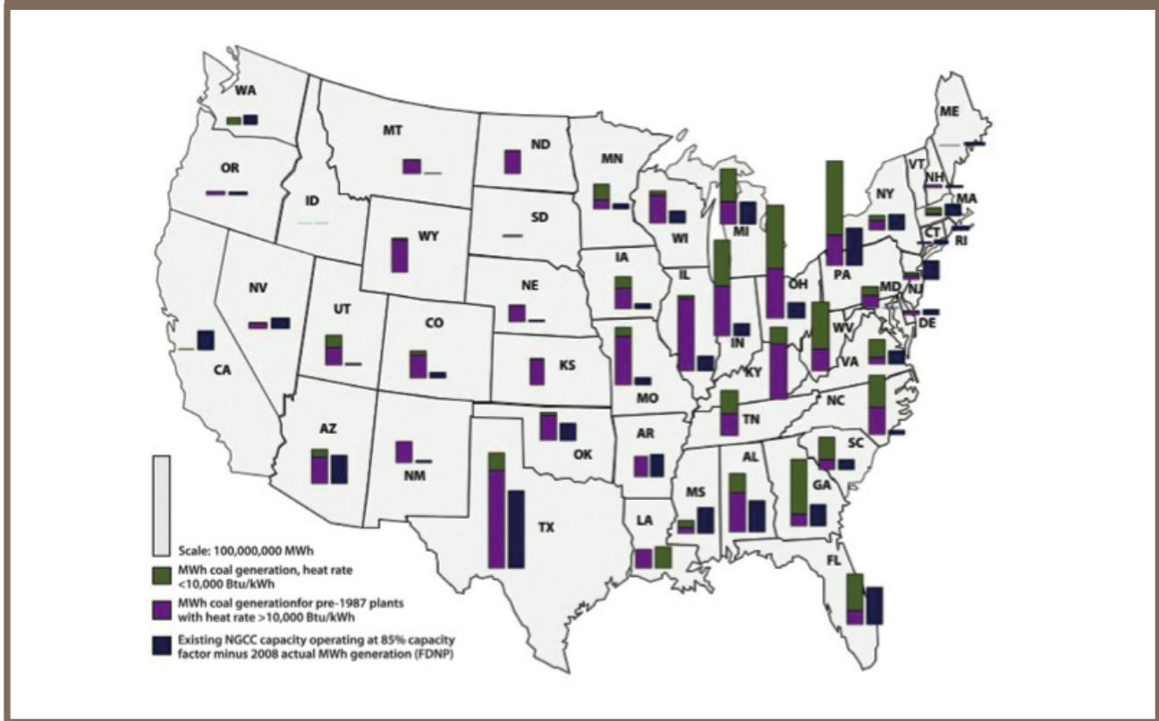
Figure 4.4 Scale and Location of Fully Dispatch NGCC Potential and Coal Generation (MWh, 2008)
