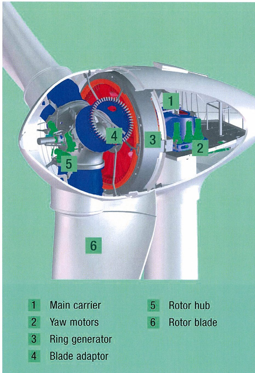
Figure 2: Illustration: Nacelle
