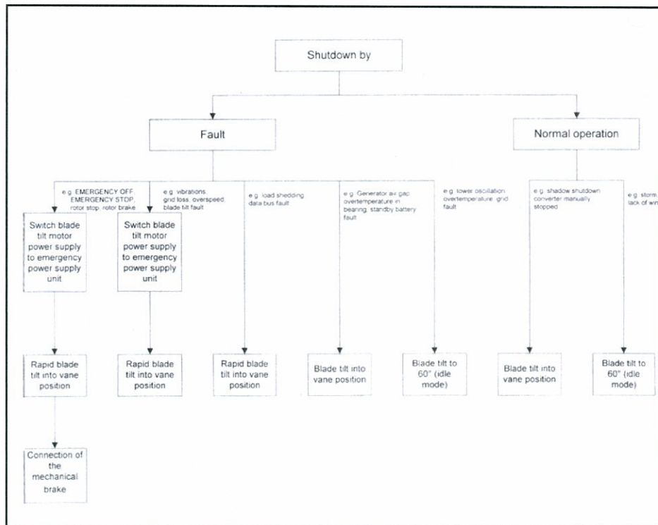
Figure 3: Shutdown procedures for the E-82
