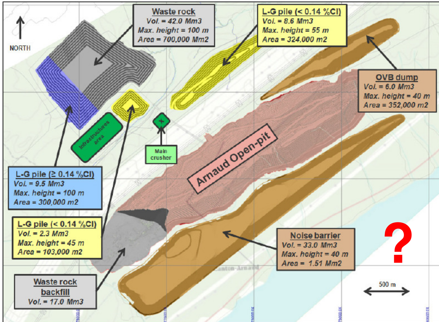
Figure 18-2: Piles locations
