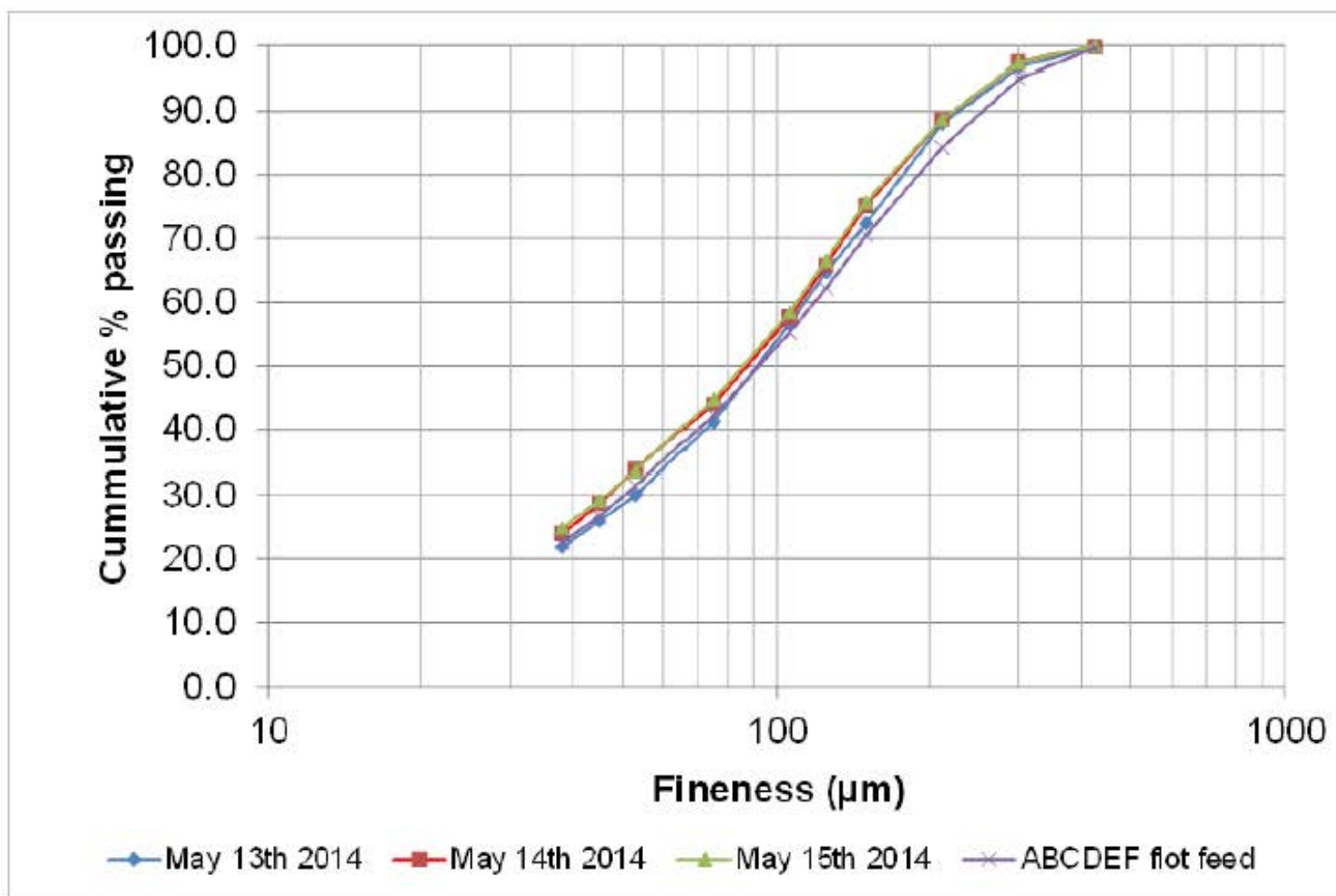
Figure 52 : Comparison between sieve distribution before and after regrinding of flotation feed for May 13 th , 14 th and 15 th 2014.
