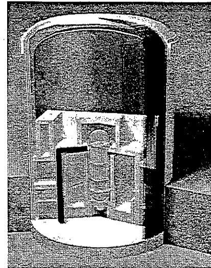
Boiling Water Reactor Containment Structure
