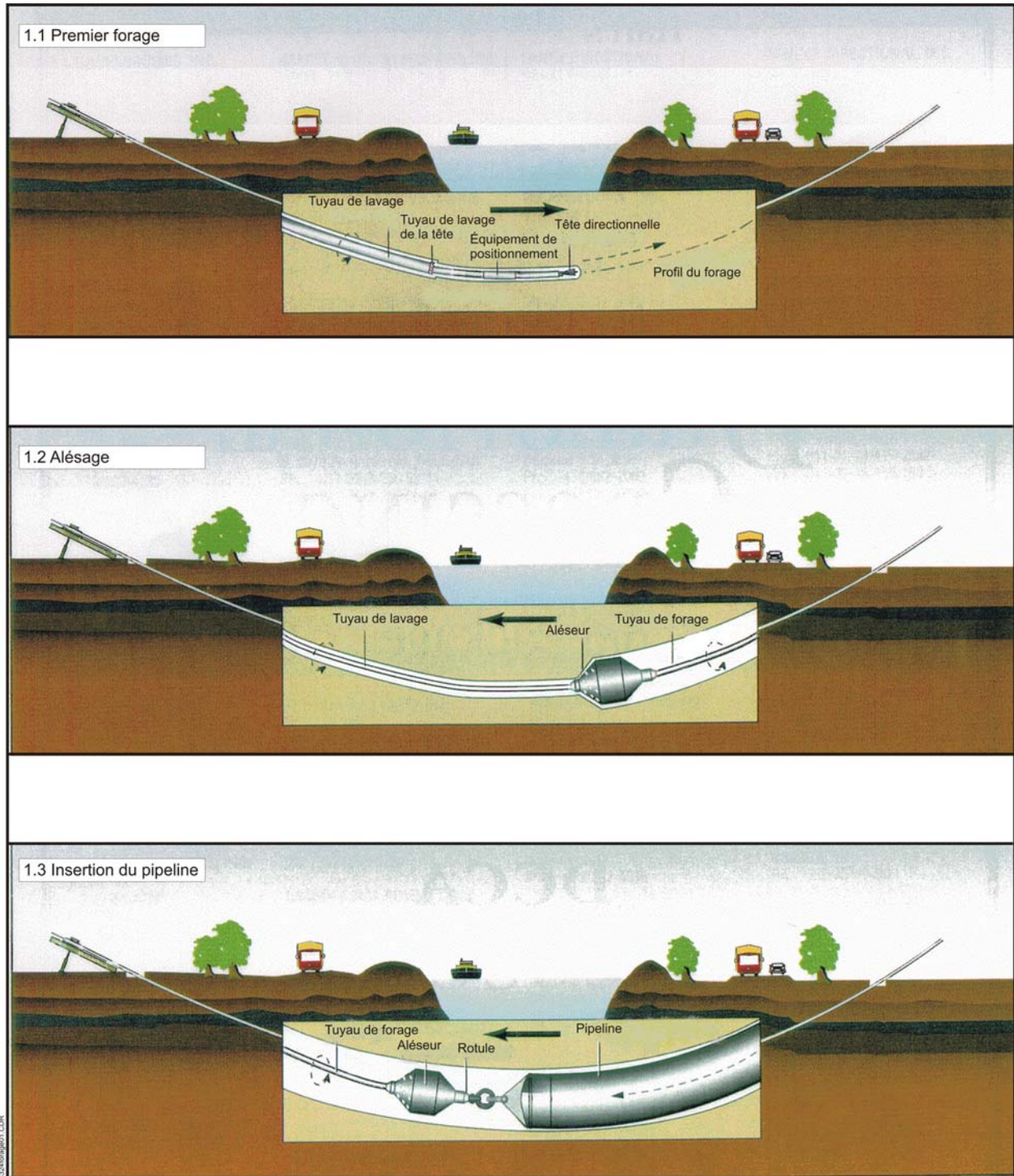
Figure 7.1 Technique de forage directionnel
