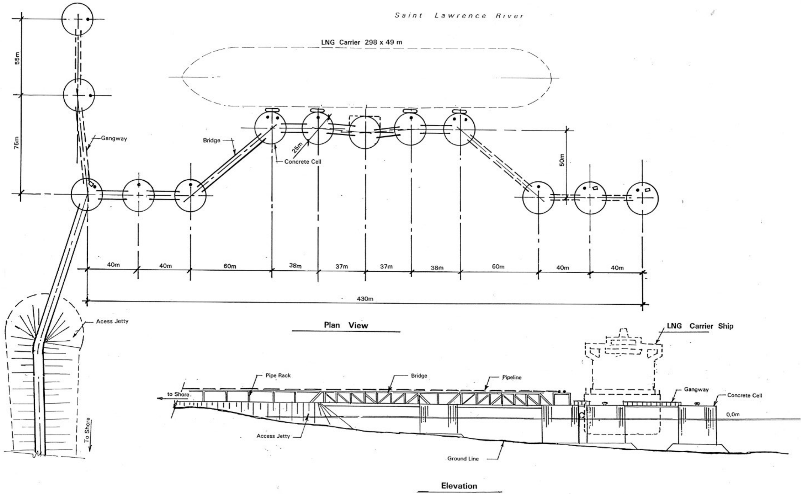
Figure 5.2 VILLE GUAY SITE GENERAL ARRANGEMENT - PLAN AND ELEVATION
