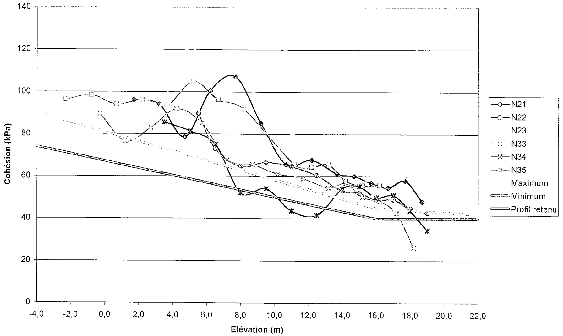
Figure 7-4-Essais Nilcon-Axes bandes
